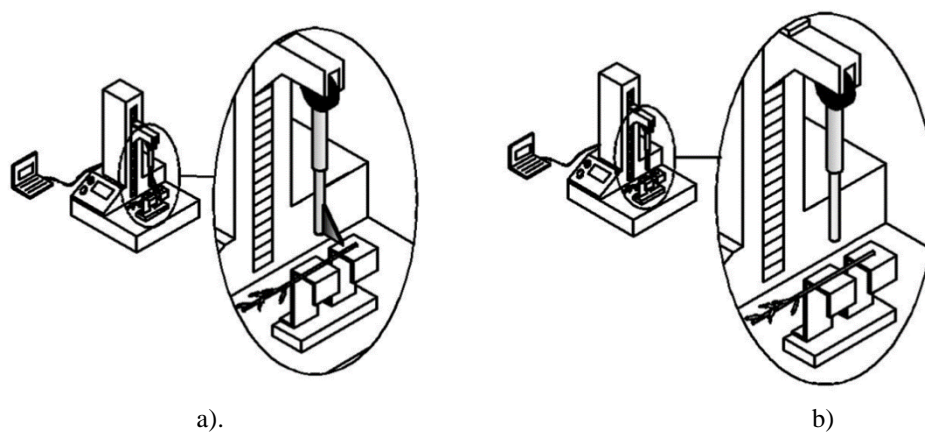
Figure 2. Computer-aided systems for measuring the cutting and bending strength of lavandin ( Lavandula x intermedia Emeric ex Loisel.) plant: a) – cutting system b) – bending system
