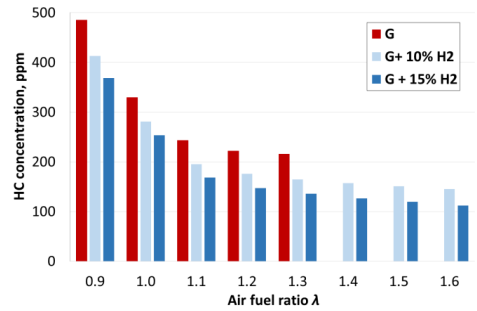
Fig. 10. Dependence of hydrocarbon concentration in combustion products on hydrogen concentration and air excess coefficient
