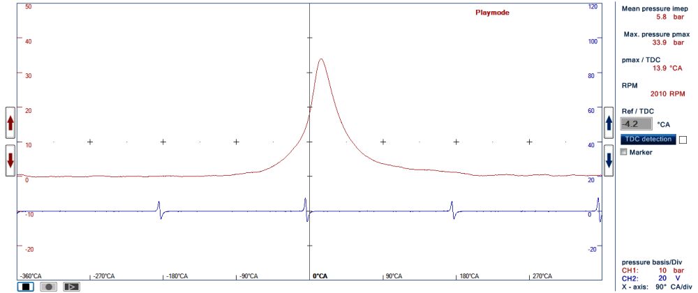
Fig. 7 Pressure in cylinder determined by stand experiments
